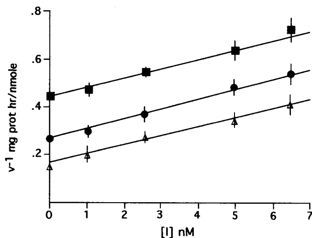
Figure 5. Dixon plot ( 1/v vs I ) for inhibition of 24-SMT by 25-thiacholesterol iodide at fixed [SAM]. Acetone powder extract of methyl transferase (1.5 mL, \sim 4 mg of protein per mL) was incubated with 400 nmol of S -methyl-[ 14 C]-SAM and 50 nmol (■), 100 nmol (●), or 200 nmol (△) of 10 at various inhibitor concentrations in a final volume of 4.0 mL at 37 °C for 30 min. Results are the average of samples from four separate experiments.
