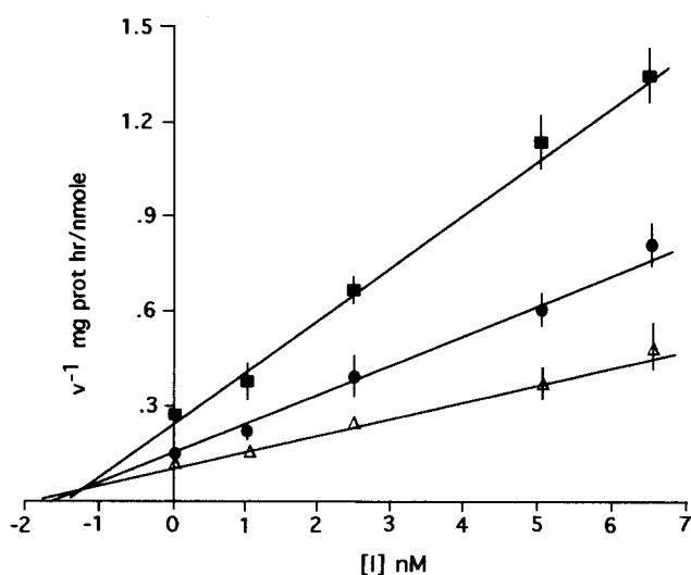
Figure 4. Dixon plot ( 1/v vs I ) for inhibition of 24-SMT by 25-thiacholesterol iodide at fixed [zymosterol]. Acetone powder extract of methyl transferase (1.5 mL, \sim 4 mg of protein per mL) was incubated with 400 nmol of 10 and 100 nmol (■), 200 nmol (●), or 400 nmol (△) of S -methyl-[ 14 C]-SAM at various inhibitor concentrations in a final volume of 4.0 mL at 37 °C for 30 min. Results are the average of samples from four separate experiments.
