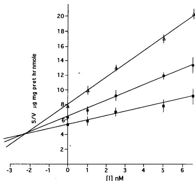
Figure 6. Plot ( s/v vs I ) for inhibition of 24-SMT by 25-thiacholesterol iodide at fixed [SAM]. Acetone powder extract of methyl transferase (1.5 mL, \sim 4 mg of protein per mL) was incubated as described in Figure 5.
